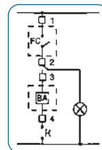
schema elettrico bobina release coil wiring scheme
