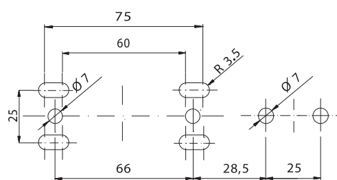
Holes for installation
