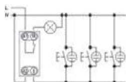
3-wire connection
